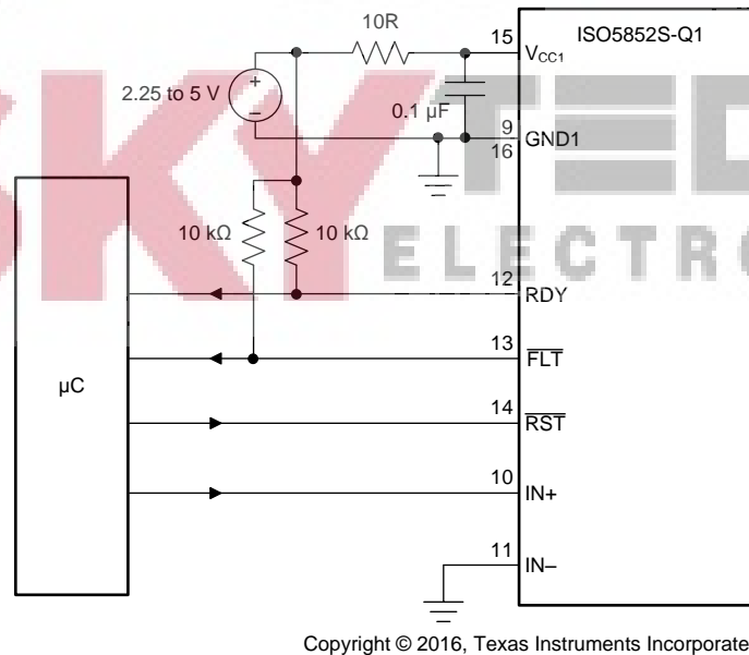
Figure 51. \overline{\text{FLT}} and RDY Pin Circuitry for High CMTI
