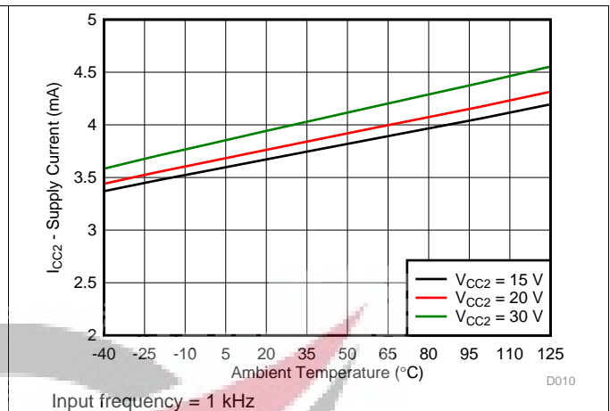
Figure 22. I CC2 Supply Current vs Temperature
