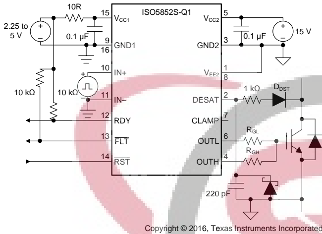
Figure 49. Unipolar Output Supply
