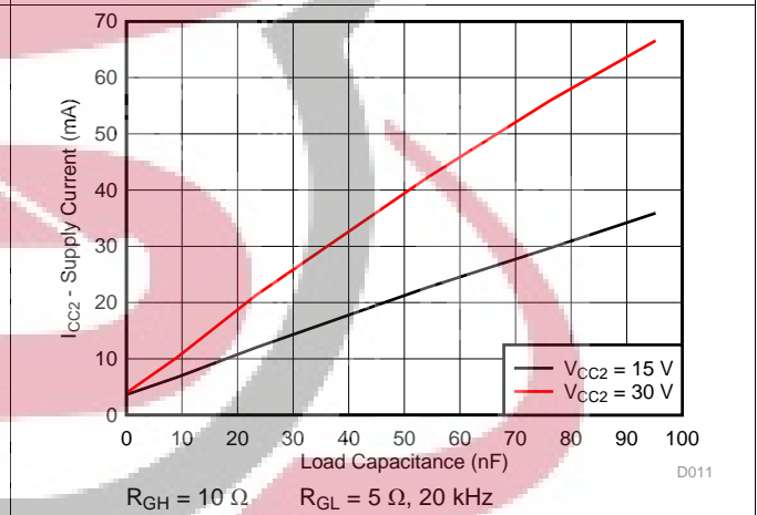
Figure 24. I CC2 Supply Current vs Load Capacitance
