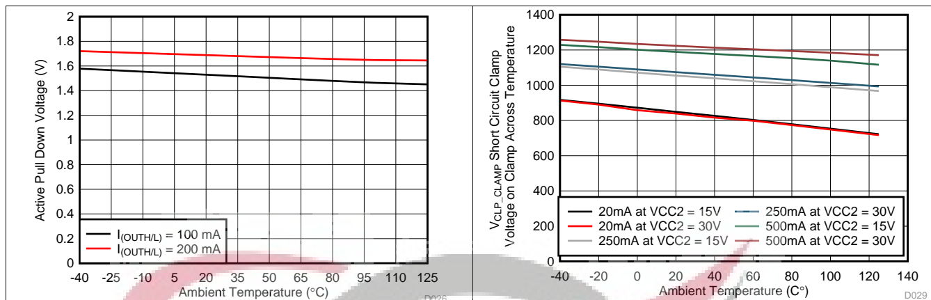
Figure 40. V_{CLP\_CLAMP} - Short-Circuit Clamp Voltage on Clamp Across Temperature
