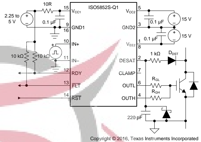
Figure 50. Bipolar Output Supply
